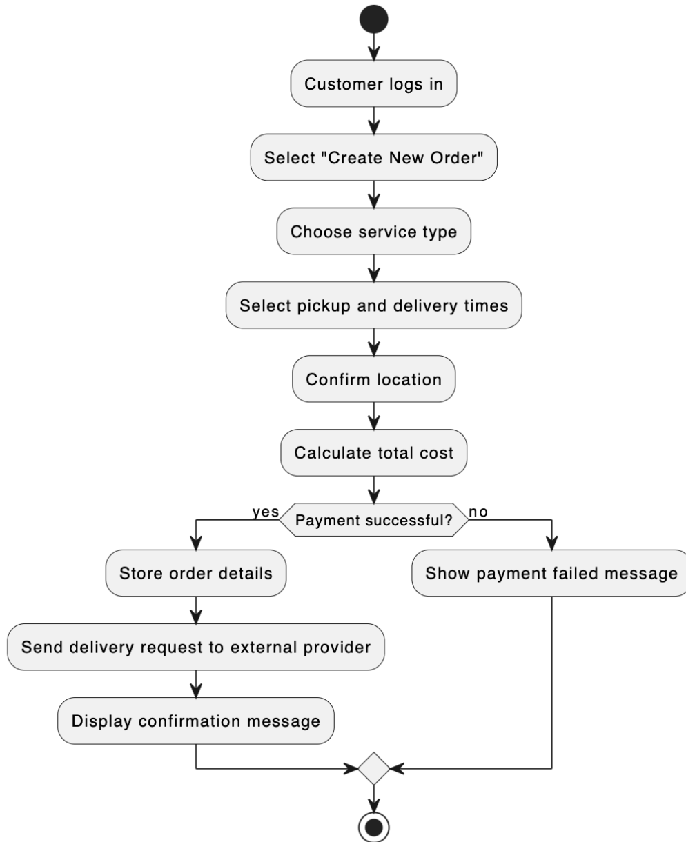
Activity Diagram for Create New Order
